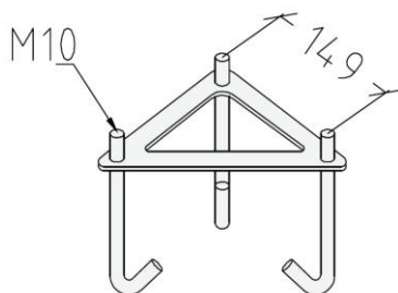
75.01556.03353 – Beton-Anker NARV
