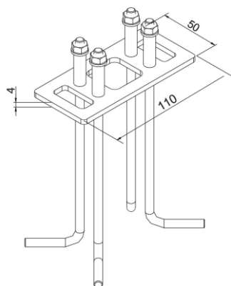
75.00285.01221 – Beton-Anker ASK, MOL
