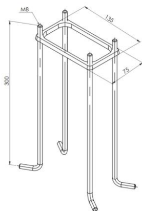
75.01554.03349 – Beton-Anker NAM
