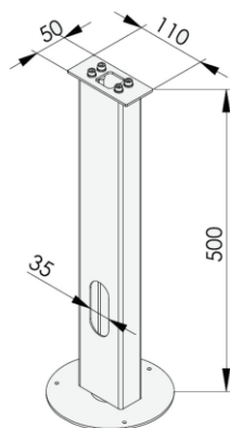
75.01559.03370 – Erdbodenhalter ASK, MOL
