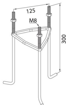
75.00287.01223 – Beton-Anker STAVA, EGER
