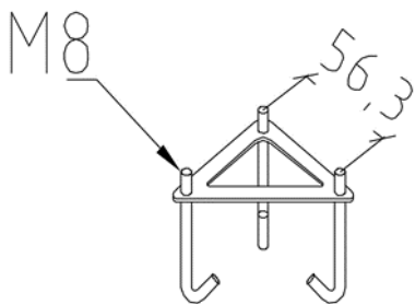
75.00286.01222 – Beton-Anker HALM, STOCK, ALT, SCAN, OPP, EGER Mini
